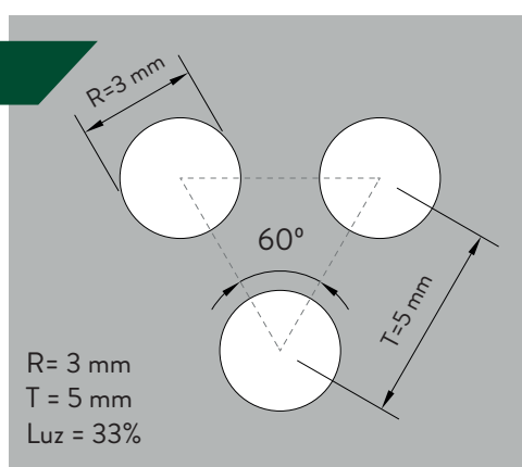
Standard drilling dimensions
