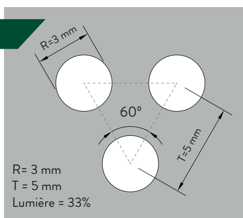
Dimensions standard des perforations
